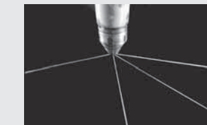
Dirty Fuel Injector Spray Pattern
